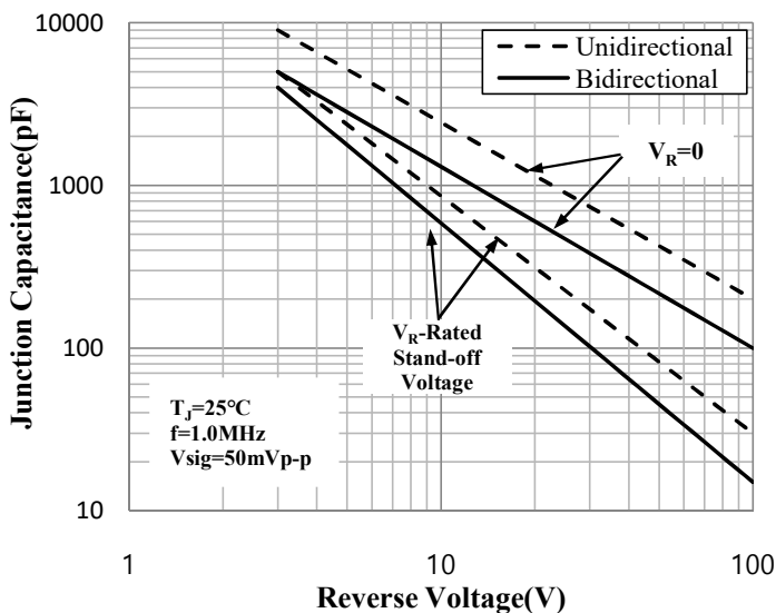
Fig. 5 Typical Junction Capacitance Unidirectional
